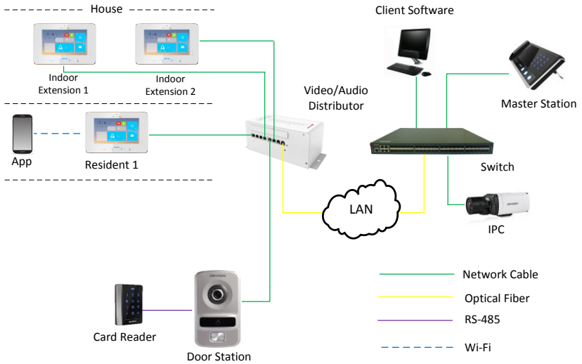
Figure 3-2 Typical Application of DS-KV8102-XP
