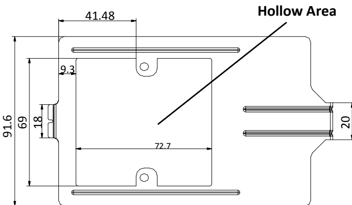
Figure 5-5 Dimensions of Installation Plate (DS-KV8102-XP)
