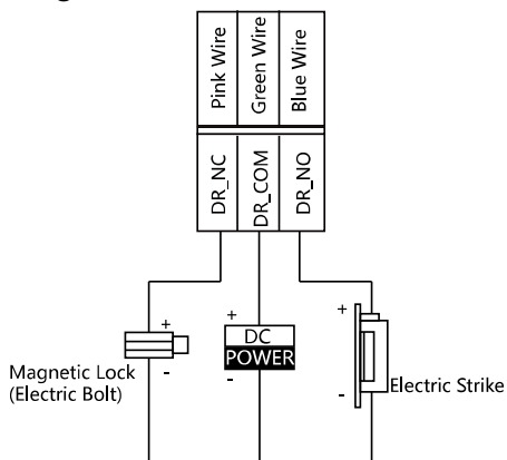
Figure 5-10 Door Lock Wiring
