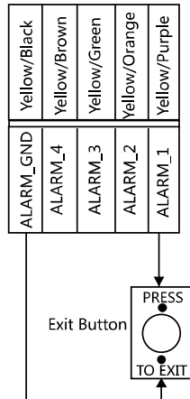
Figure 5-12 Exit Button Wiring
